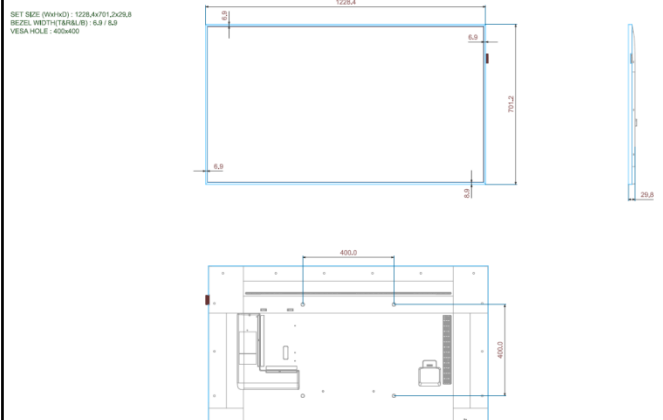
PMF/PHF 55inch Mechanical Drawing_160204
