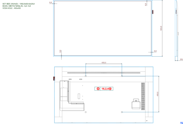
PMF/PHF 49inch Mechanical Drawing_160204
