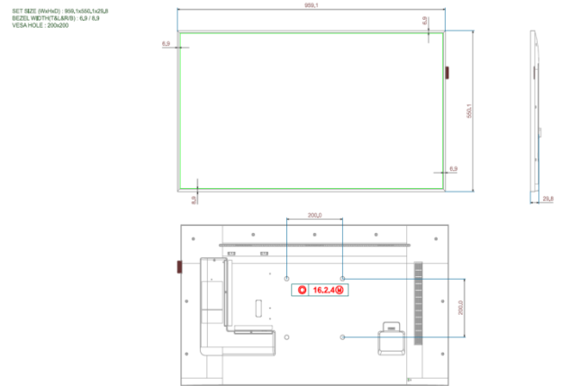
PMF/PHF 43inch Mechanical Drawing_160204
